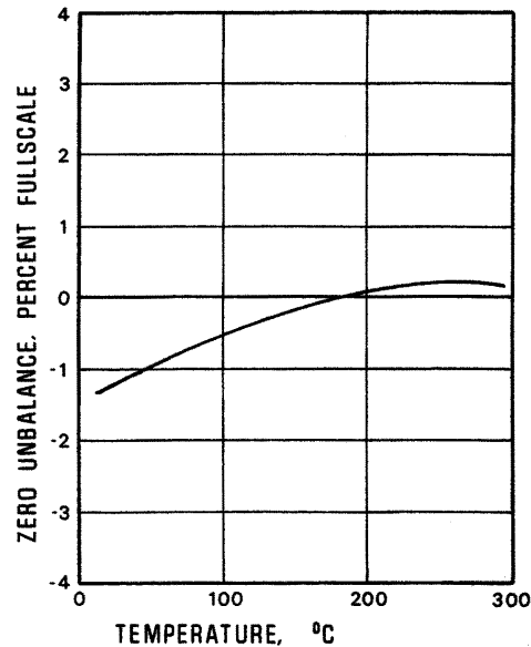
Figure 7. Zero Compensation
