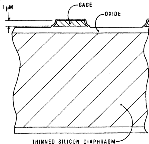
Figure 3. Oxide-Bonded Gage
