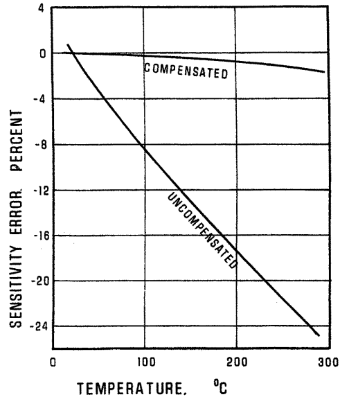
Figure 6. Sensitivity Compensation
