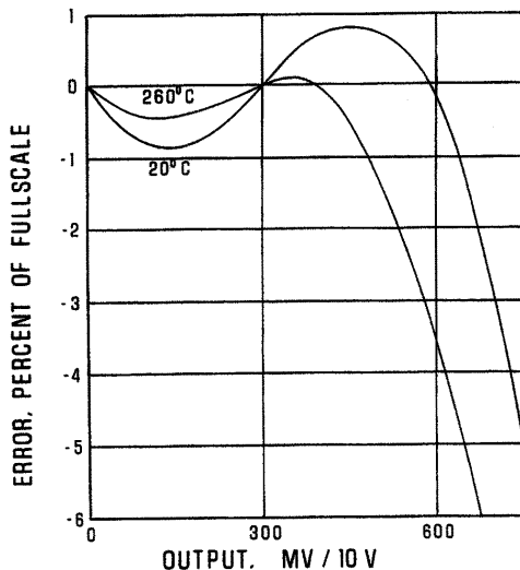
Figure 5. Nonlinearity
