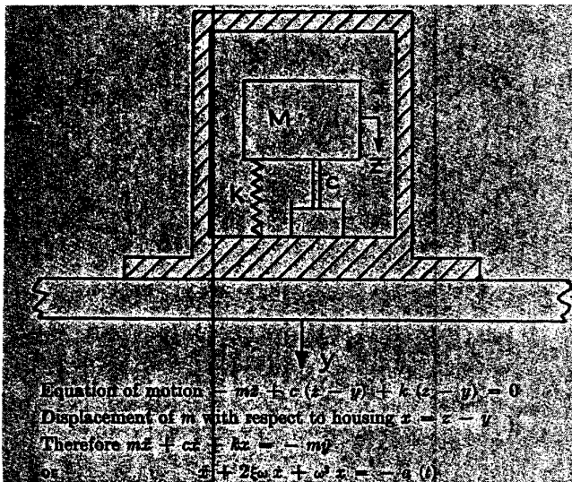
Fig. 1: Almost all accelerometers are like the one shown here. The basic equations associated with this unit are listed below.
