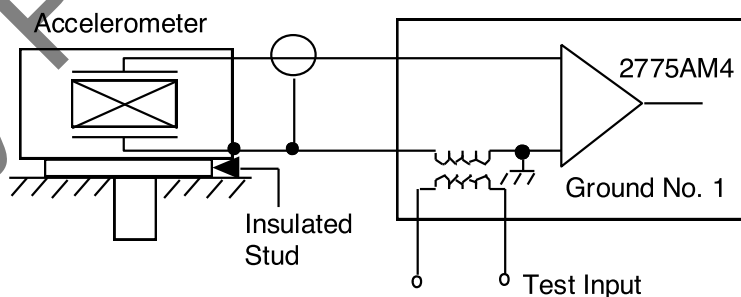
FIGURE 3-5: TEST INPUT
