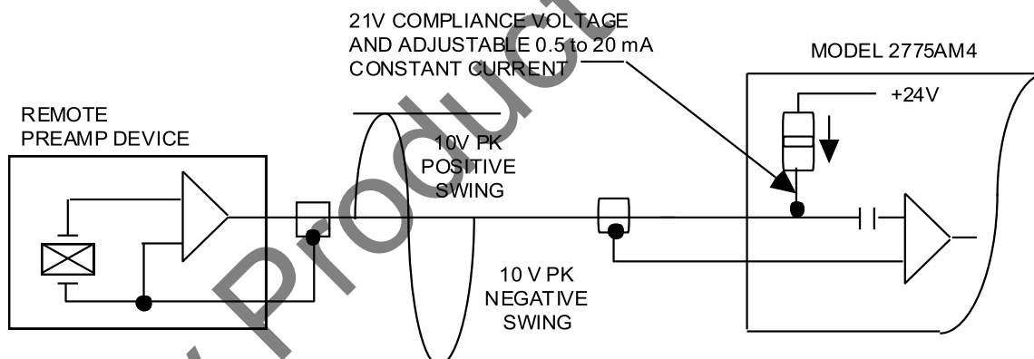
FIGURE 3-7: REMOTE HOOKUP
