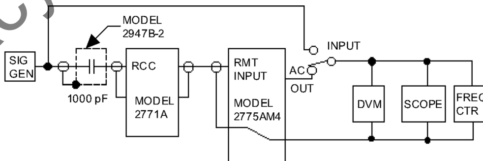
FIGURE 6-6: 2771A/2775AM4 TEST SETUP
